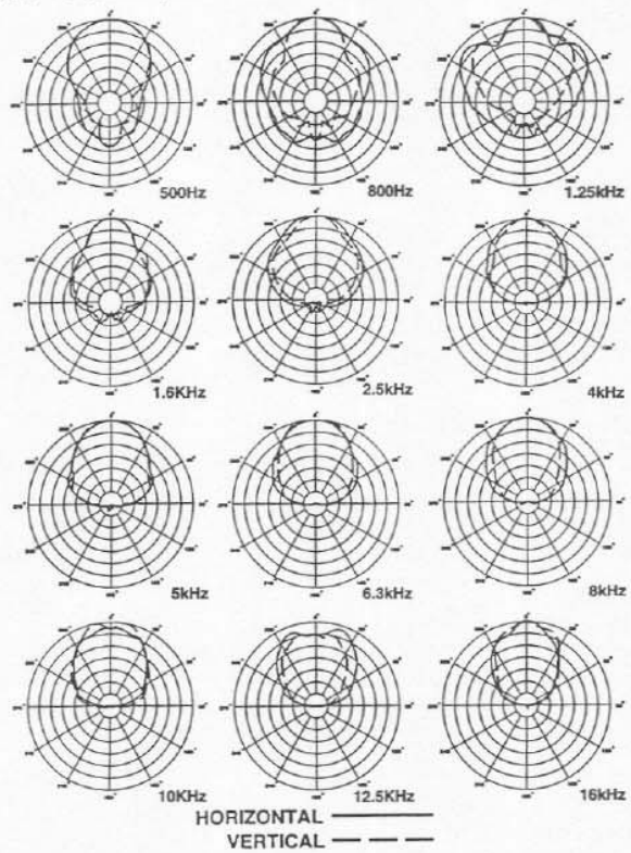
FIGURE 6 — Polar Response
